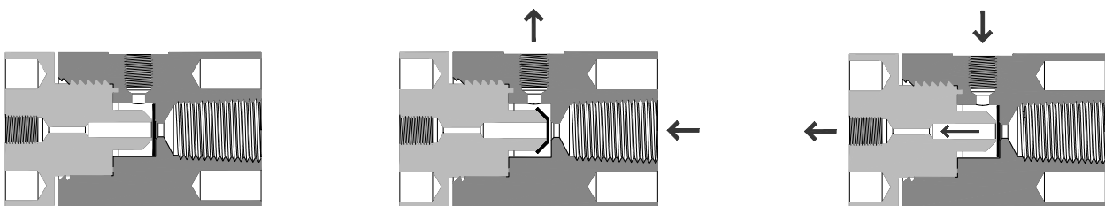
Valve at rest
